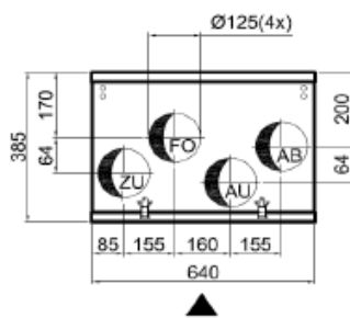
EA180.6 Bypass links
